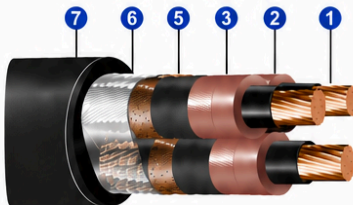
Three-core (Multiple)
